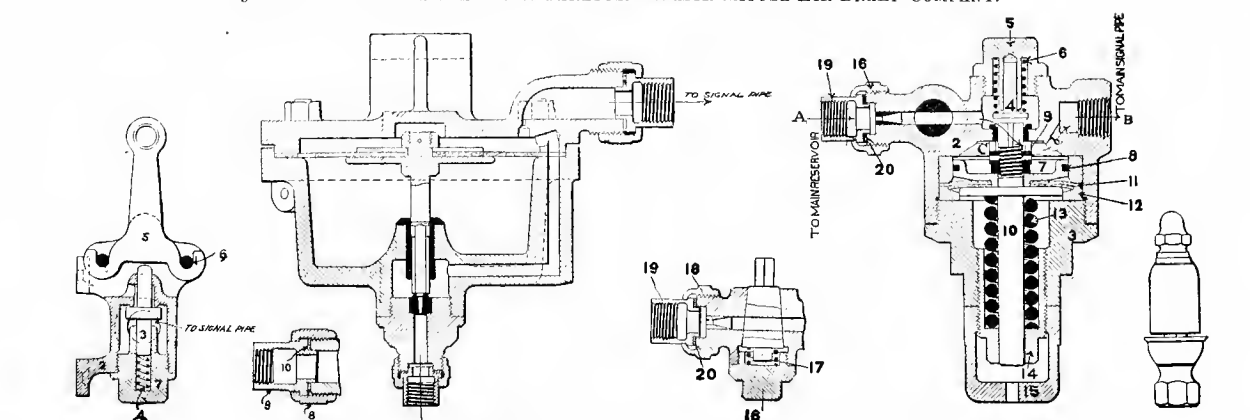
Fig. 2402. Car Discharge-valve.
